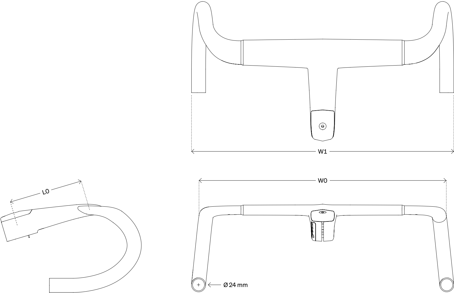
WO/W1 Misurata esterno-esterno WO/W1 Measured outside-outside
